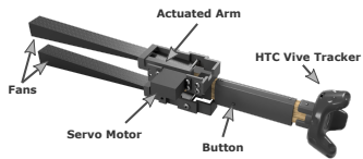
Figure 3: 3D rendering of the Drag:on prototype.
